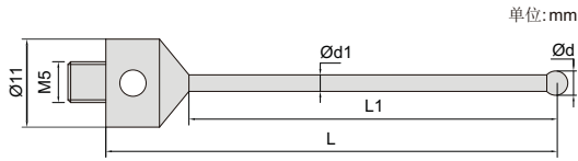
M5测针(不锈钢基座)
