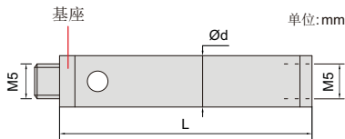
M5测针延长杆
